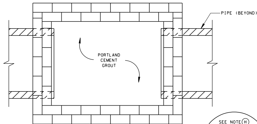
SECTION E-E
